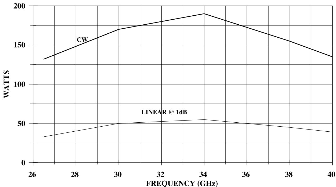
130T26z5G40B TYPICAL POWER OUTPUT
