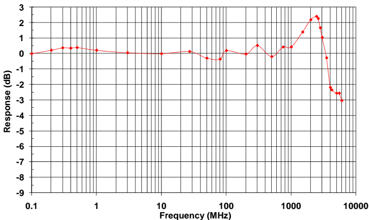
FL7006CC Typical Uncalibrated Frequency Response
