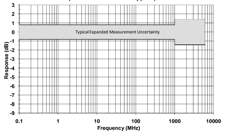
FL7006CC Typical Calibrated Frequency Response (with correction factors applied)
