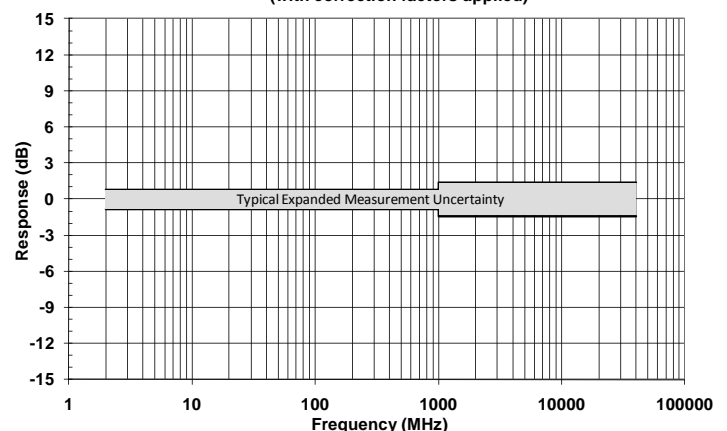
FL7040CC Typical Calibrated Frequency Response (with correction factors applied)
