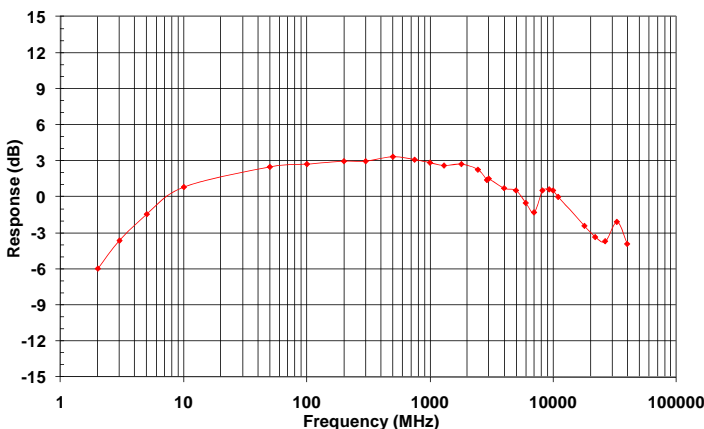
FL7040CC Typical Uncalibrated Frequency Response
