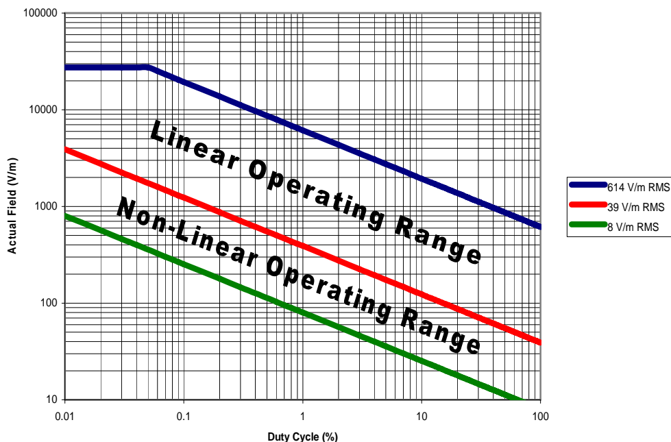
FP7050 Operating Limits
