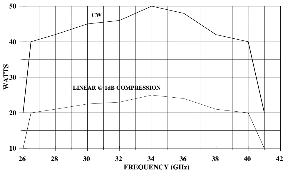
40T26G40A TYPICAL POWER OUTPUT
